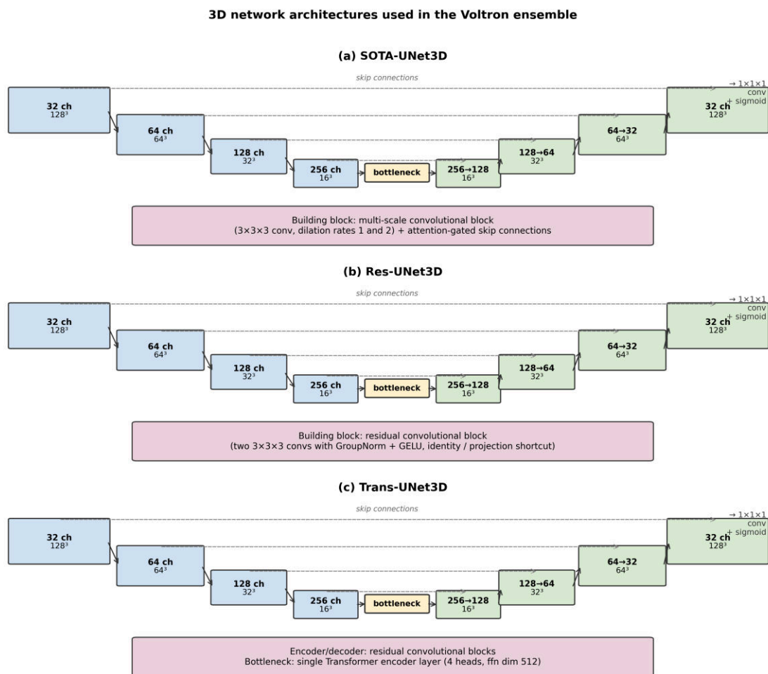
Supplementary Fig. S2. Schematic of the three three-dimensional networks that make up the Voltron ensemble. All three share a four-level encoder–decoder topology with skip connections; they differ in the type of computational block applied at each stage. (a) SOTA-UNet3D uses multi-scale convolutional blocks (dilated 3 \times 3 \times 3 convolutions with dilation rates 1 and 2) combined with attention-gated skip connections. (b) Res-UNet3D uses simple residual convolutional blocks (two 3 \times 3 \times 3 convolutions with group normalisation and
